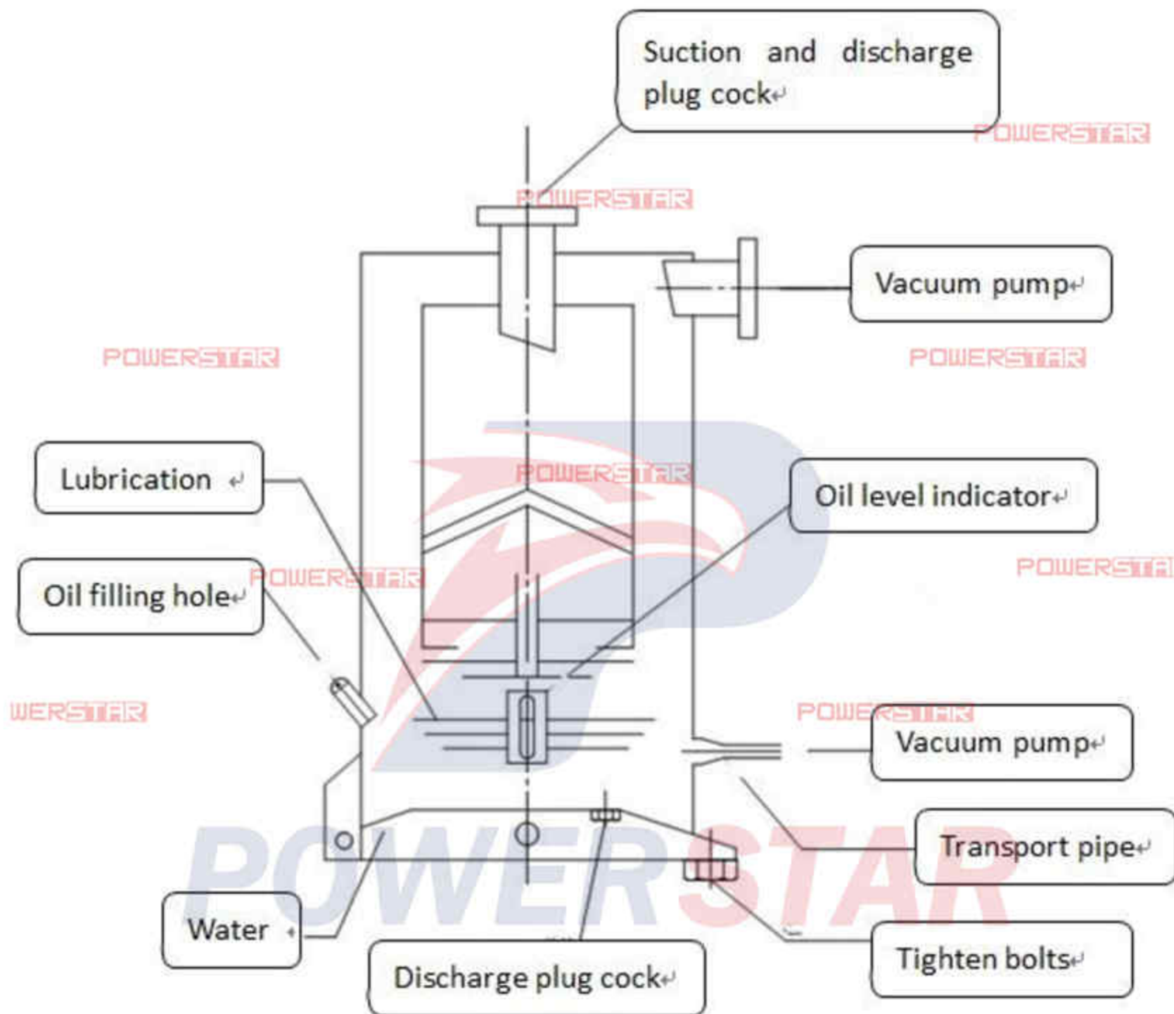
(Second Level Oil-Gas Separator)
