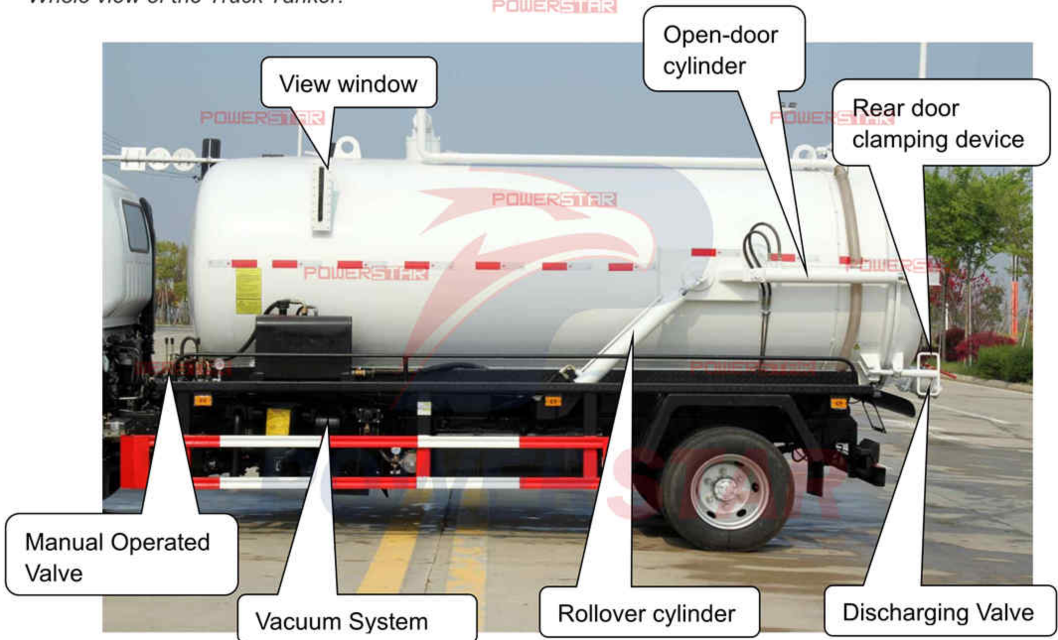
Whole view of the Truck Tanker:
